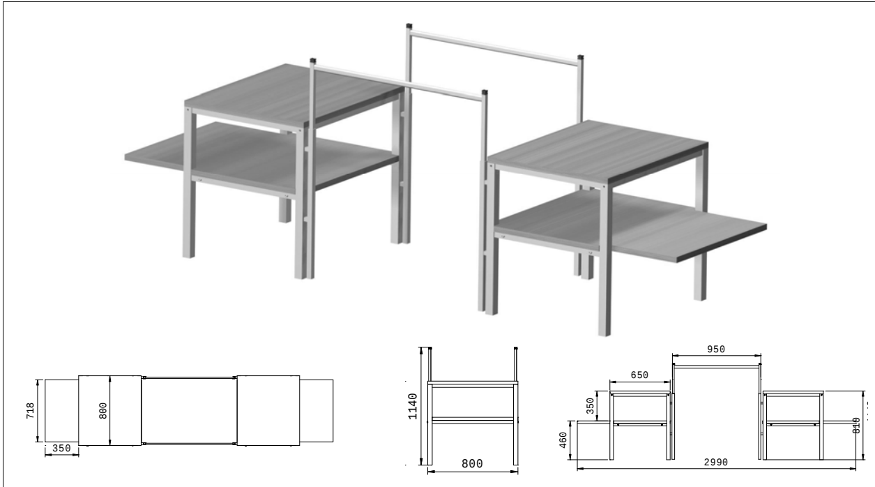
KATLI MASA TİP 1 MULTI LAYERED TABLE TYPE 1 U012 0011 00
