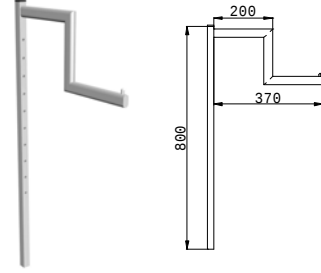
KOL TİP-2 / HANGER TYPE 2
