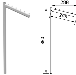
KOL TİP-3 / HANGER TYPE 3
