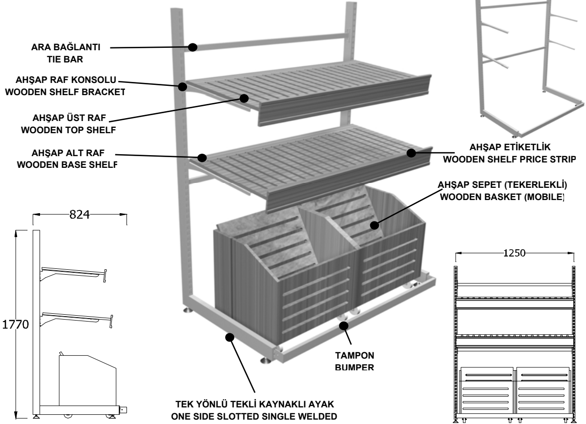
UM8 UNLU MAMUL REYONU UM8 BAKERY UNIT
